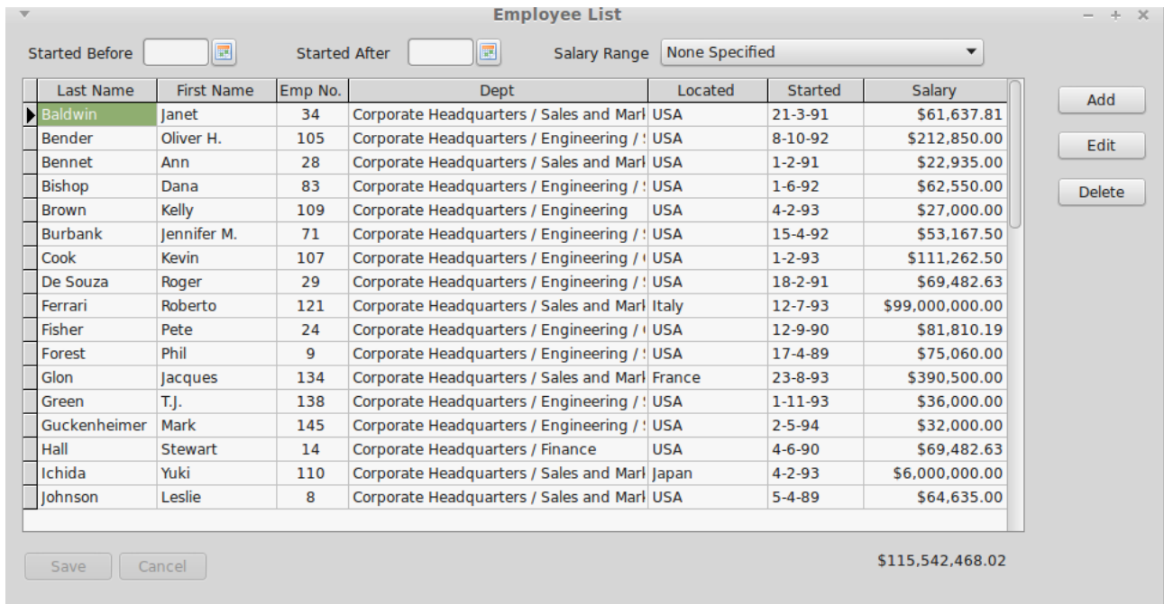
Illustration 8: The TIBDynamicGrid
