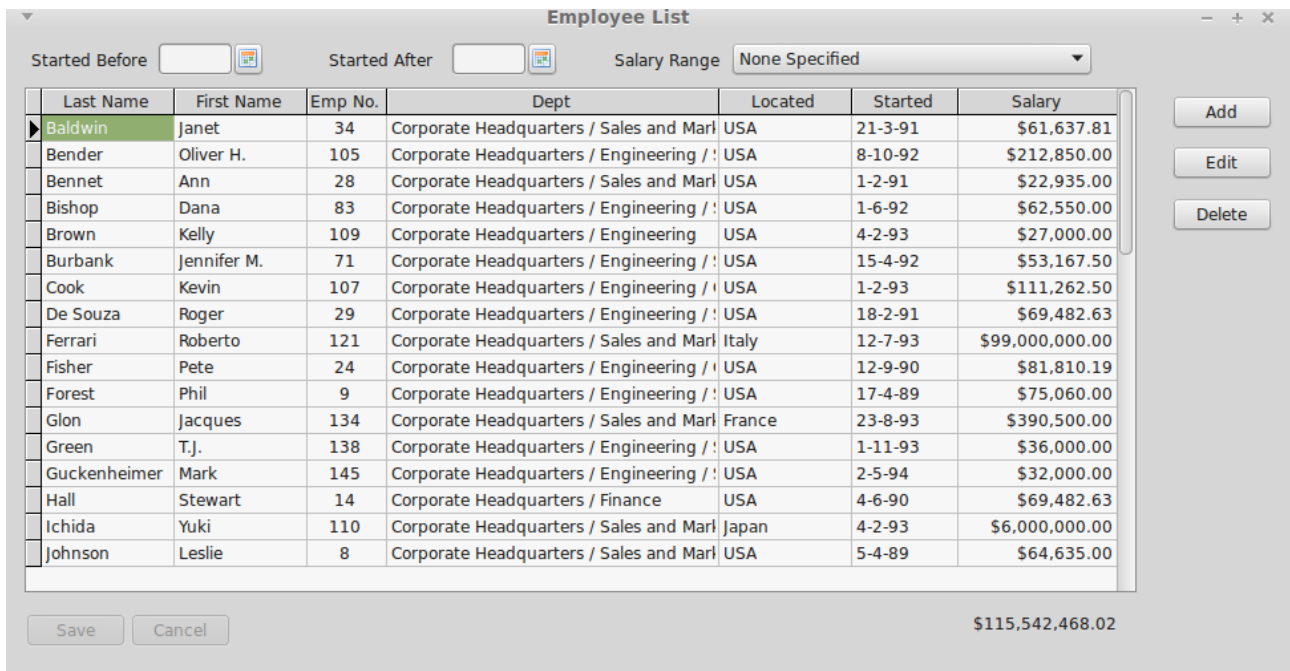
Illustration 11: The TIBDynamicGrid
